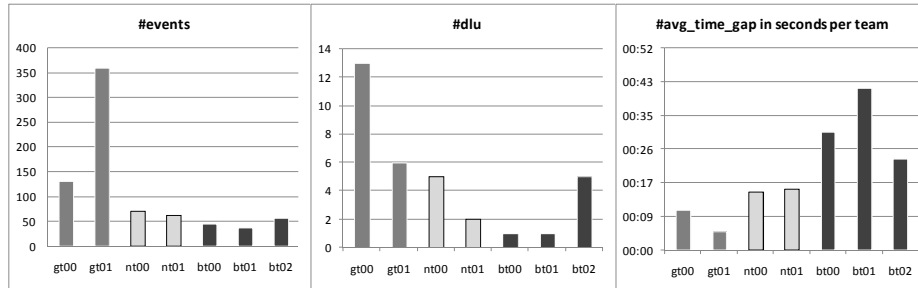
Fig. 1. Total sum of events ( #events ), difference of ( #link actions - #unlink actions ) ( #dlu ) and average time between consecutive actions ( #avg_time_gap ) for good, neutral, bad teams (gt, nt, bt) as calculated from the logfiles of the application
