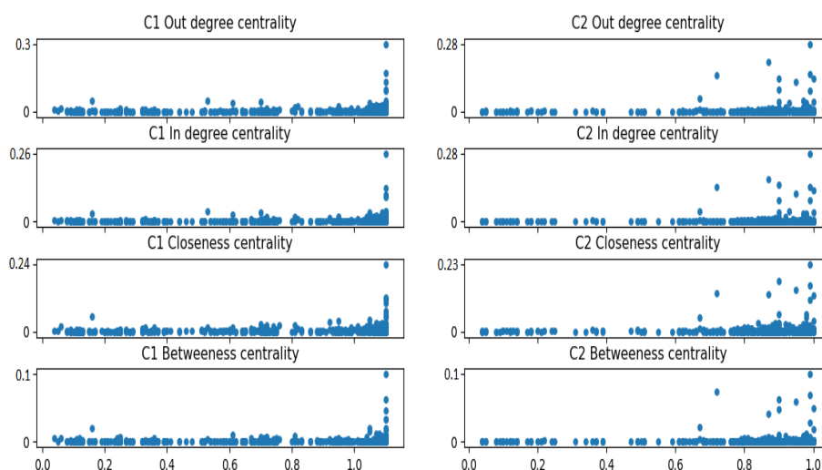
Figure 5: Scatter plots for centrality vs final grade for the two courses
